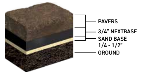
NEXTBASE™ METHOD (Approx. 3" of excavation)
