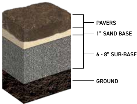
TRADITIONAL METHOD (Approx. 9 - 11" of excavation)
