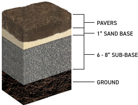
TRADITIONAL METHOD (Approx. 9 - 11" of excavation)
